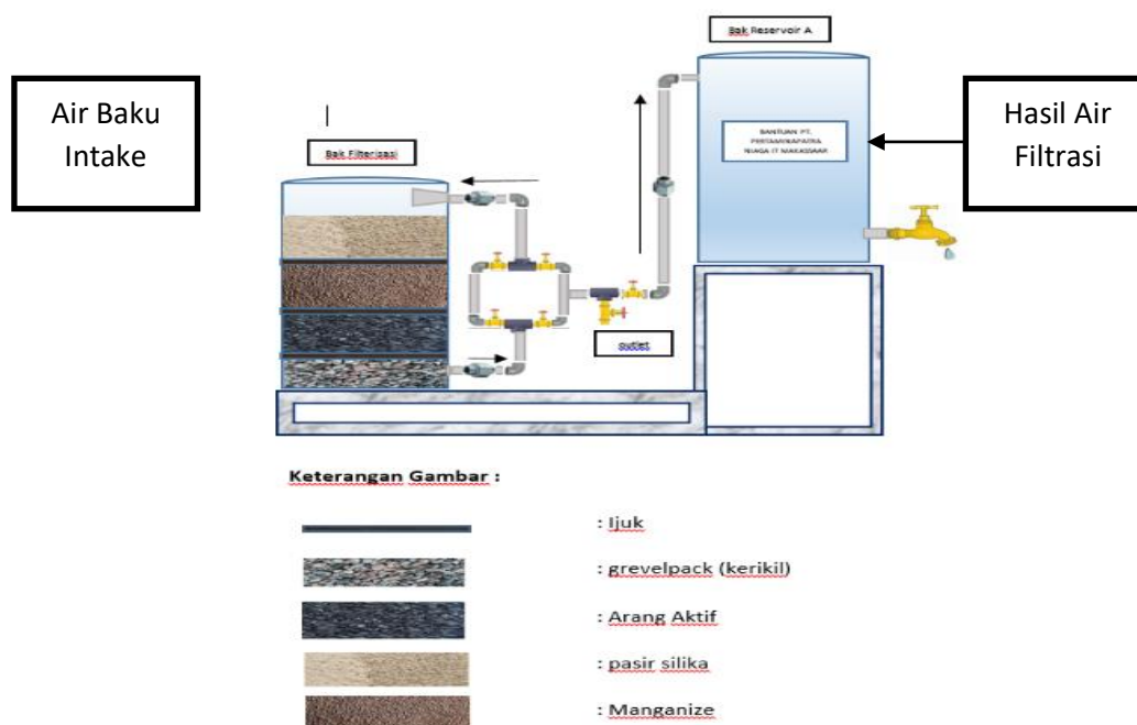
Gambar 2. Media Filter
